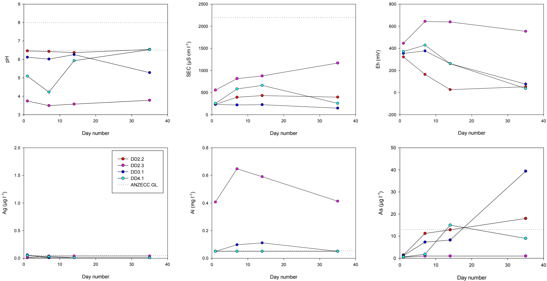
Figure 3-1 Contaminant and metalloid dynamics results for Devon Downs North wetland soil materials for pH, SEC, Eh, silver (Ag), aluminium (Al) and arsenic (As).
