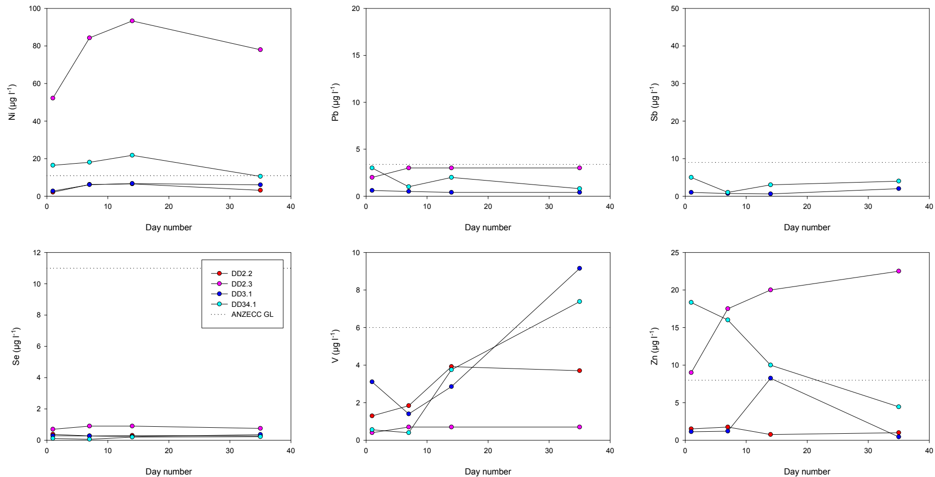
Figure 3-3 Contaminant and metalloid dynamics results for Devon Downs North wetland soil materials for nickel (Ni), lead (Pb), antimony (Sb), selenium (Se), vanadium (V) and zinc (Zn).
