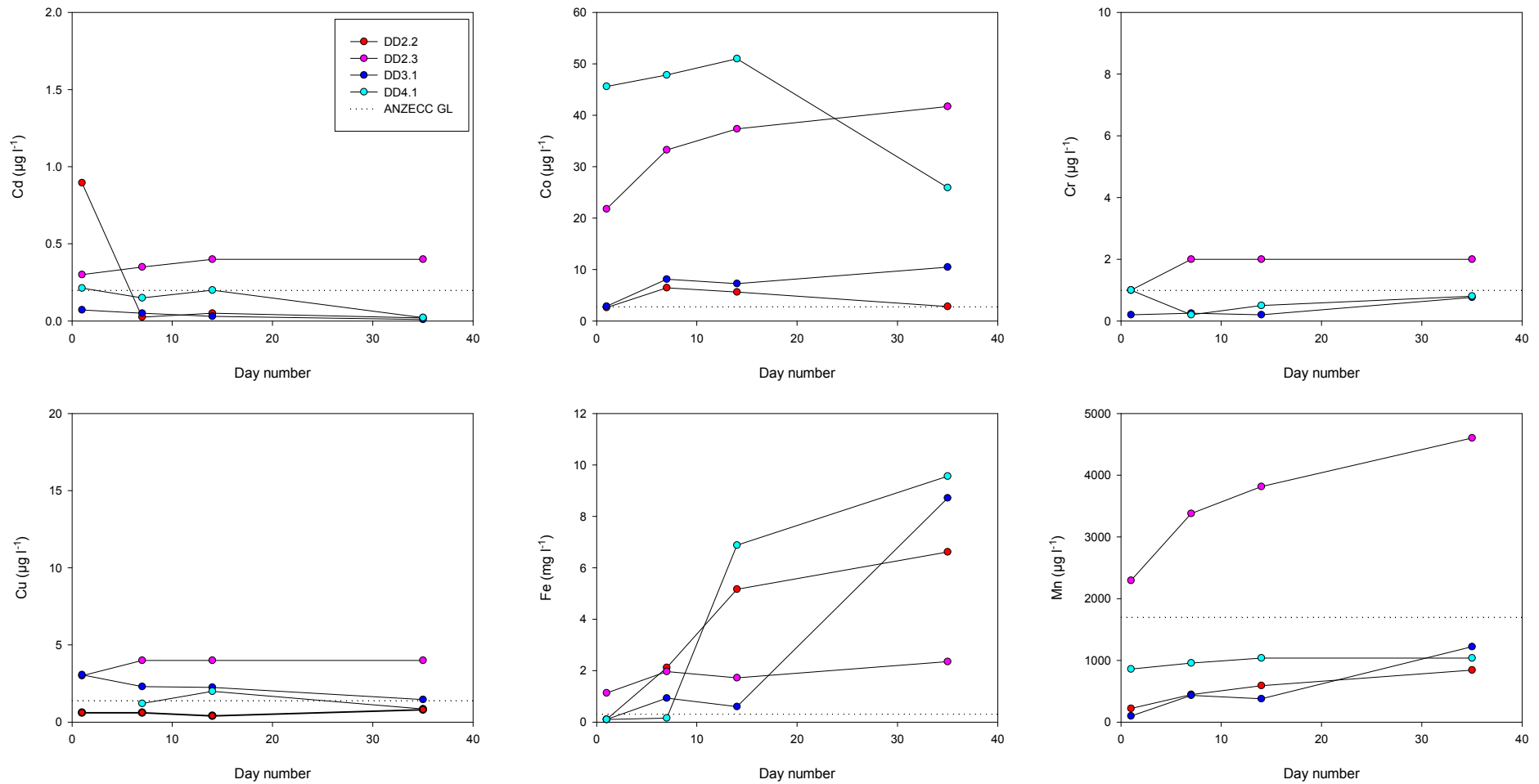
Figure 3-2 Contaminant and metalloid dynamics results for Devon Downs North wetland soil materials for cadmium (Cd), cobalt (Co), chromium (Cr), copper (Cu), iron (Fe) and manganese (Mn).
