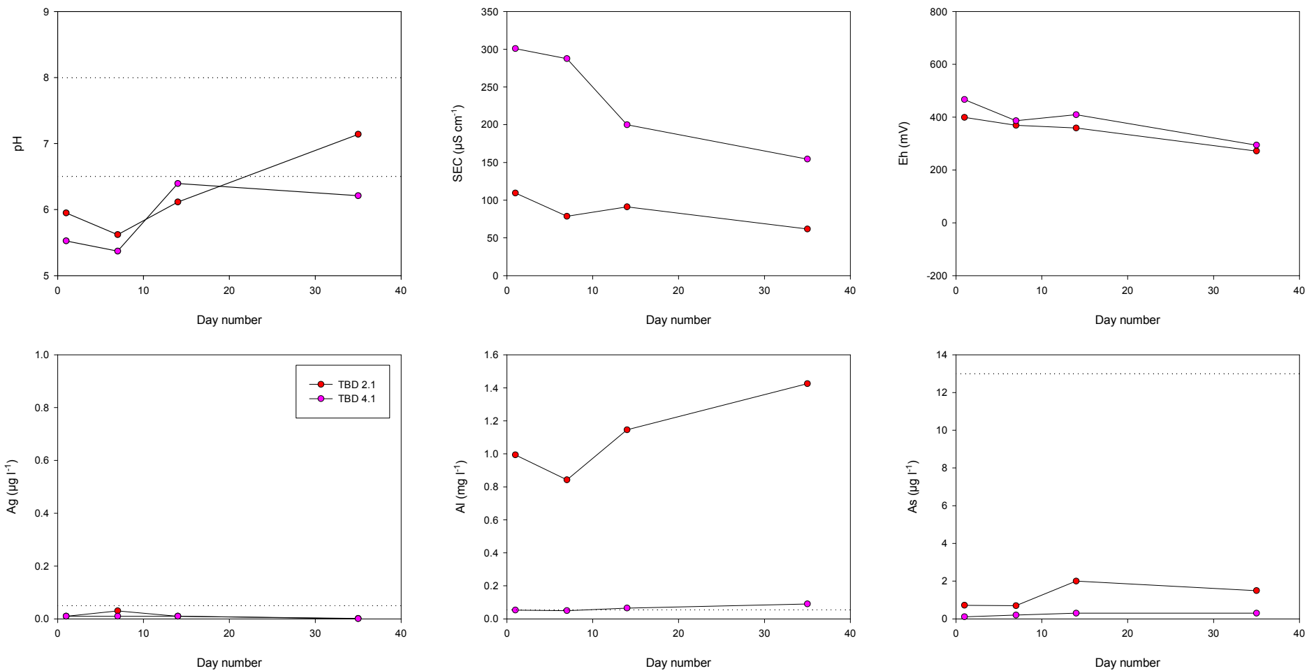
Figure 3-1 Contaminant and metalloid dynamics results for Taillem Bend wetland soil materials for pH, SEC, Eh, silver (Ag), aluminium (Al) and arsenic (As).
