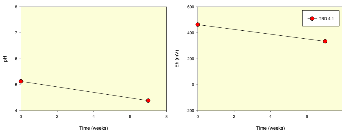
Figure 3-5 pH and Eh dynamics during monosulfide formation potential tests in surface soil sample TBD 4.1 from Taillem Bend wetland.
