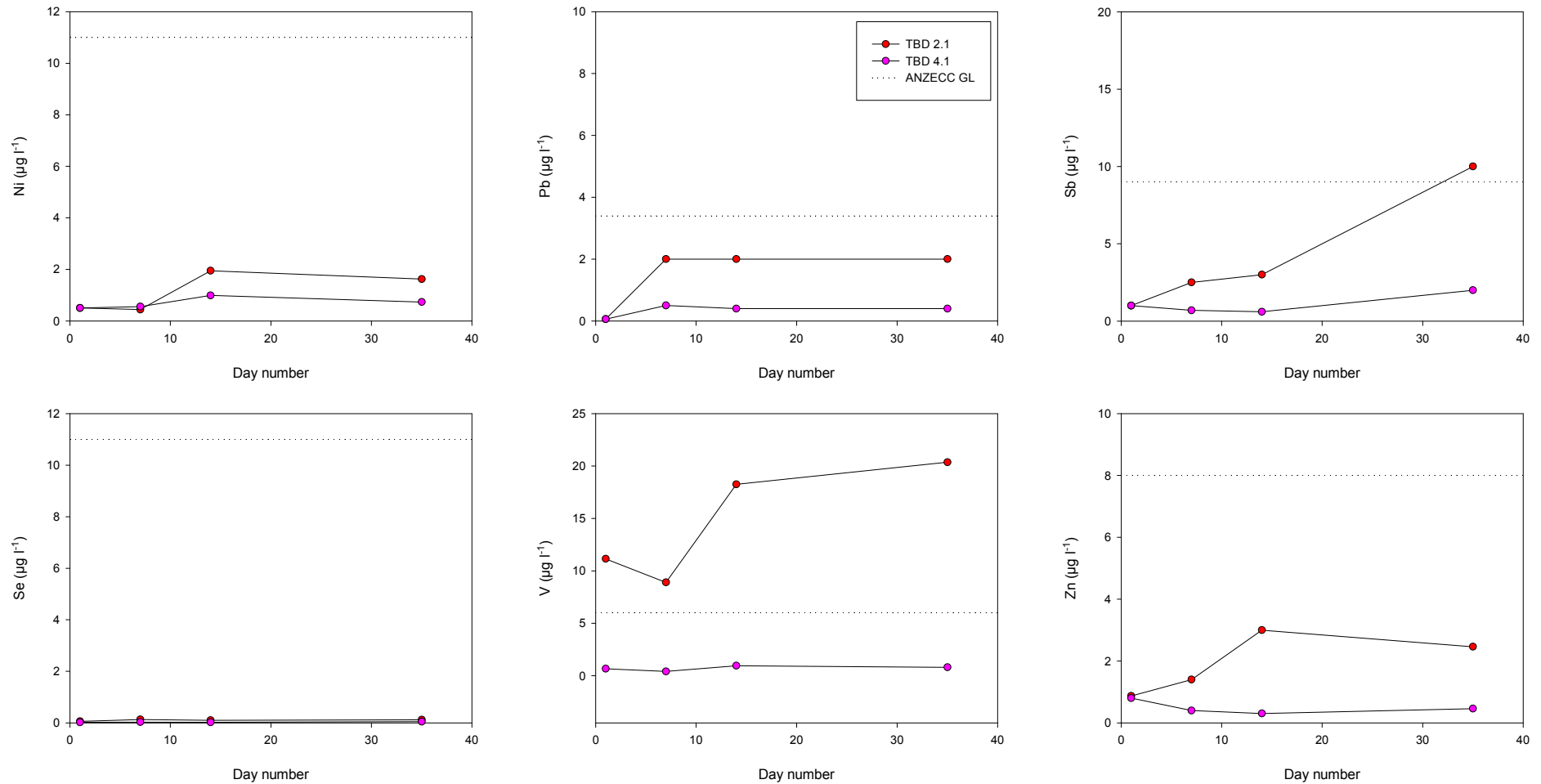
Figure 3-3 Contaminant and metalloid dynamics results for Taillem Bend wetland soil materials for nickel (Ni), lead (Pb), antimony (Sb), selenium (Se), vanadium (V) and zinc (Zn).
