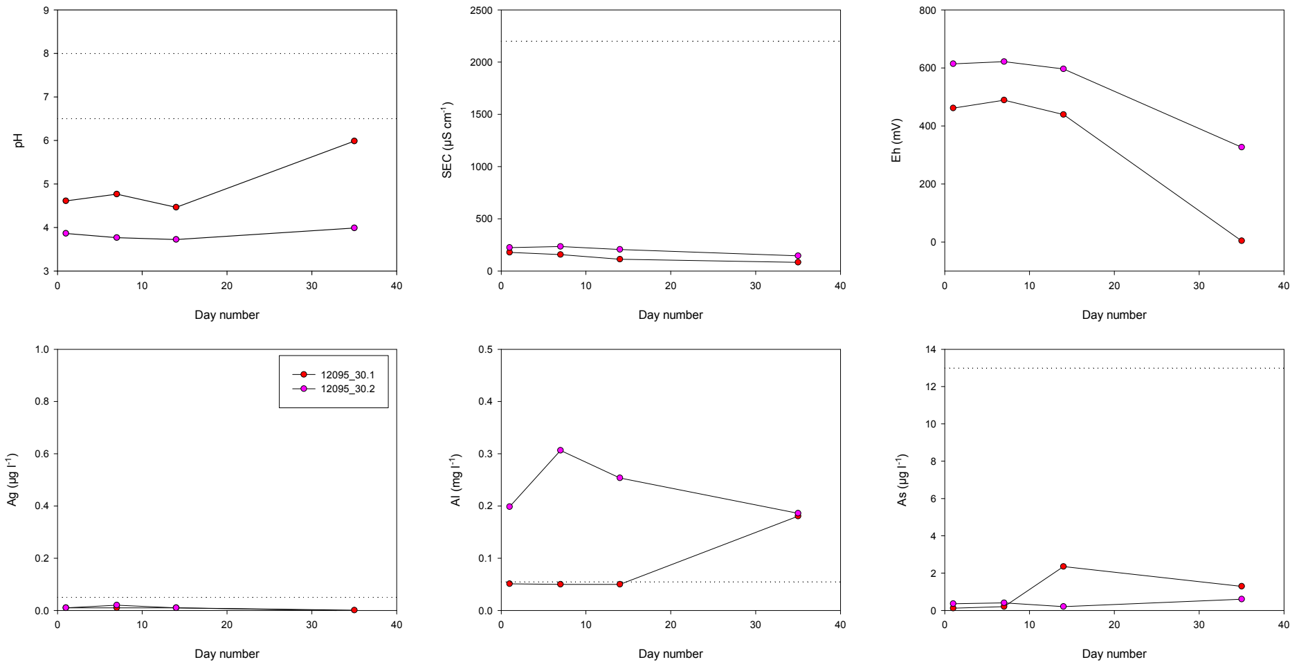
Figure 3-1 Contaminant and metalloid dynamics results for Berri Disposal Basin (12095) wetland soil materials for pH, SEC, Eh, silver (Ag), aluminium (Al) and arsenic (As).
