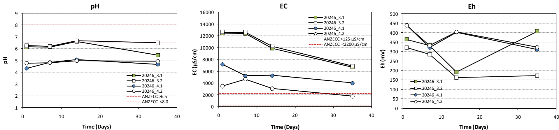
Figure 3-1: pH, EC and Eh dynamics over 35 days for the Wakool River Billabong sites (20246_3 and 20246_4).
