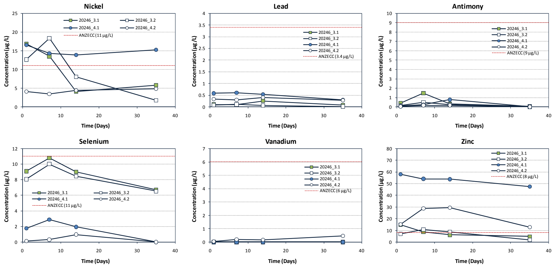
Figure 3-4: Contaminant and metalloid dynamics (Ni, Pb, Sb, Se, V and Zn) dynamics over 35 days the Wakool River Billabong sites (20246_3 and 20246_4).
