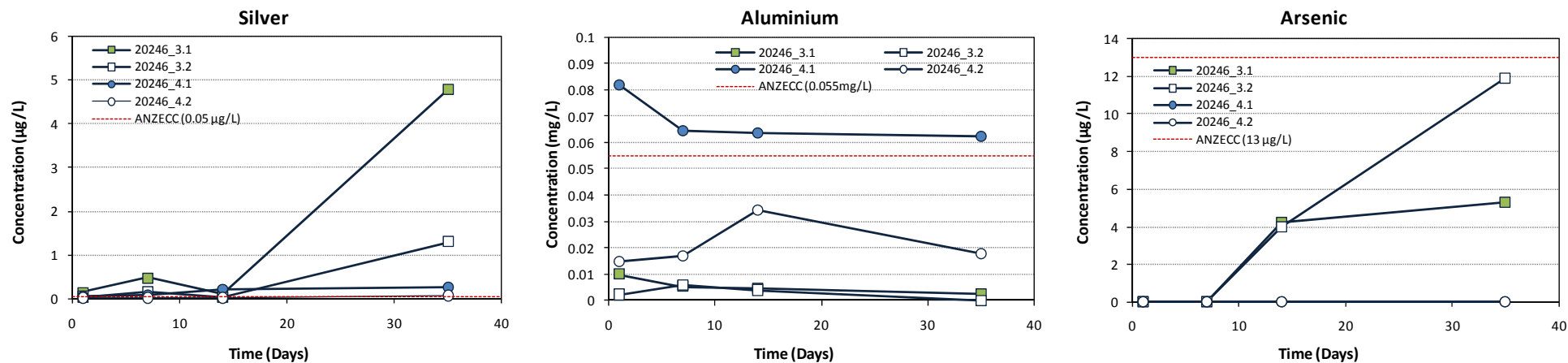
Figure 3-2: Contaminant and metalloid dynamics (Ag, Al and As) over 35 days for the Wakool River Billabong sites (20246_3 and 20246_4).
