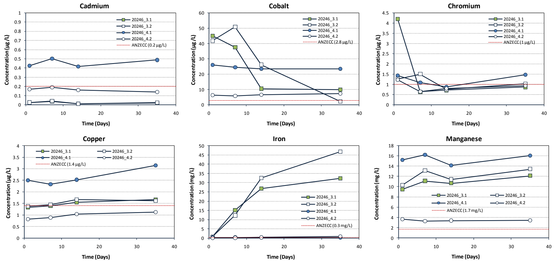
Figure 3-3: Contaminant and metalloid dynamics (Cd, Co, Cr, Cu, Fe and Mn) over 35 days the Wakool River Billabong sites (20246_3 and 20246_4).
