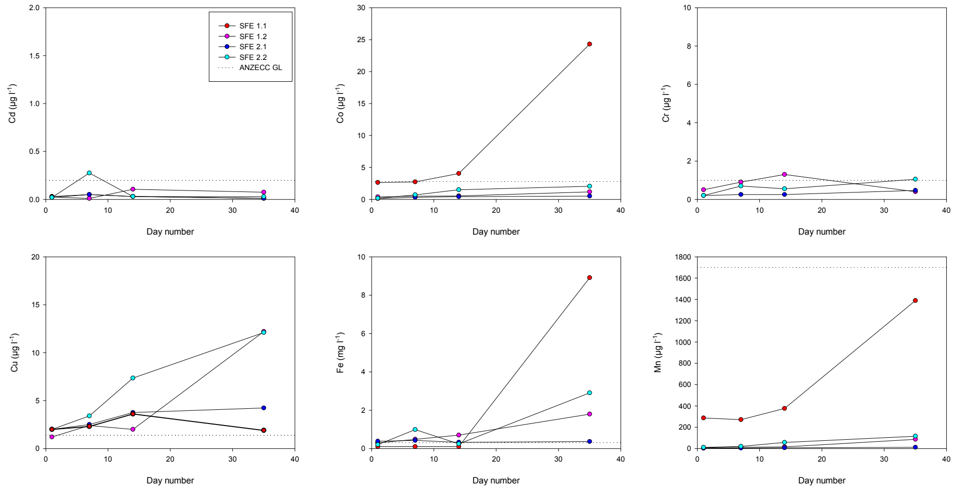
Figure 3-2 Contaminant and metalloid dynamics results for Swan Reach Ferry wetland soil materials for cadmium (Cd), cobalt (Co), chromium (Cr), copper (Cu), iron (Fe) and manganese (Mn).
