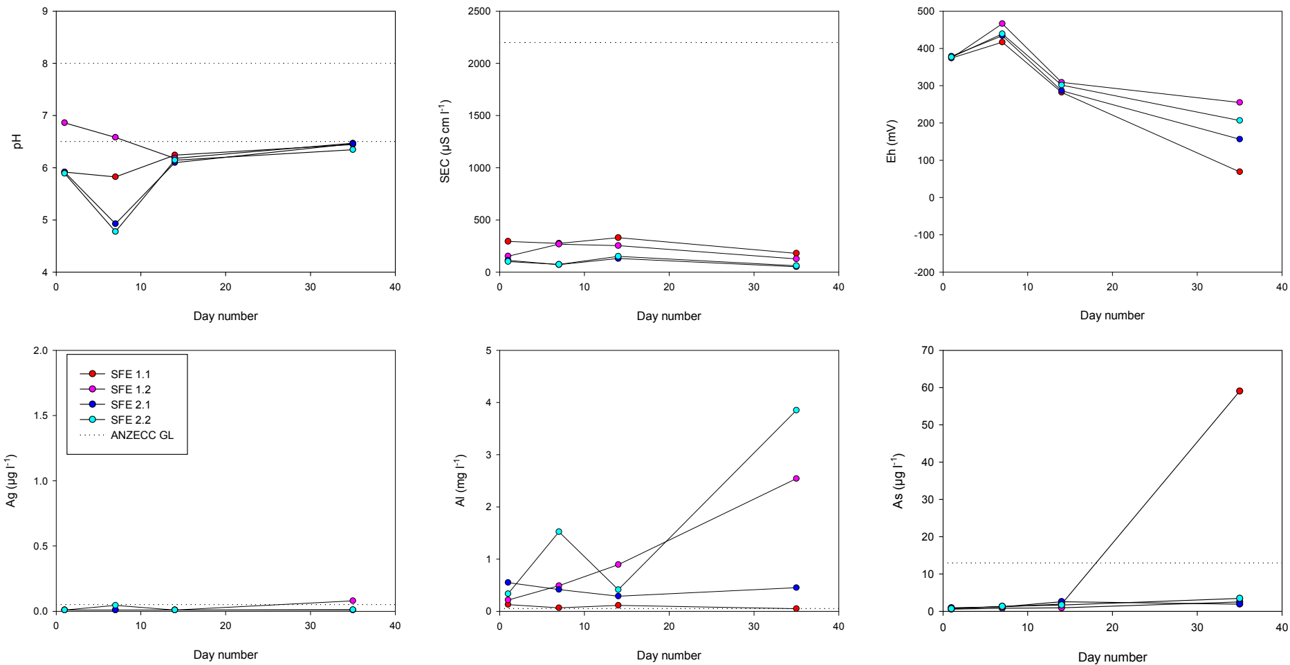
Figure 3-1 Contaminant and metalloid dynamics results for Swan Reach Ferry wetland soil materials for pH, SEC, Eh, silver (Ag), aluminium (Al) and arsenic (As).
