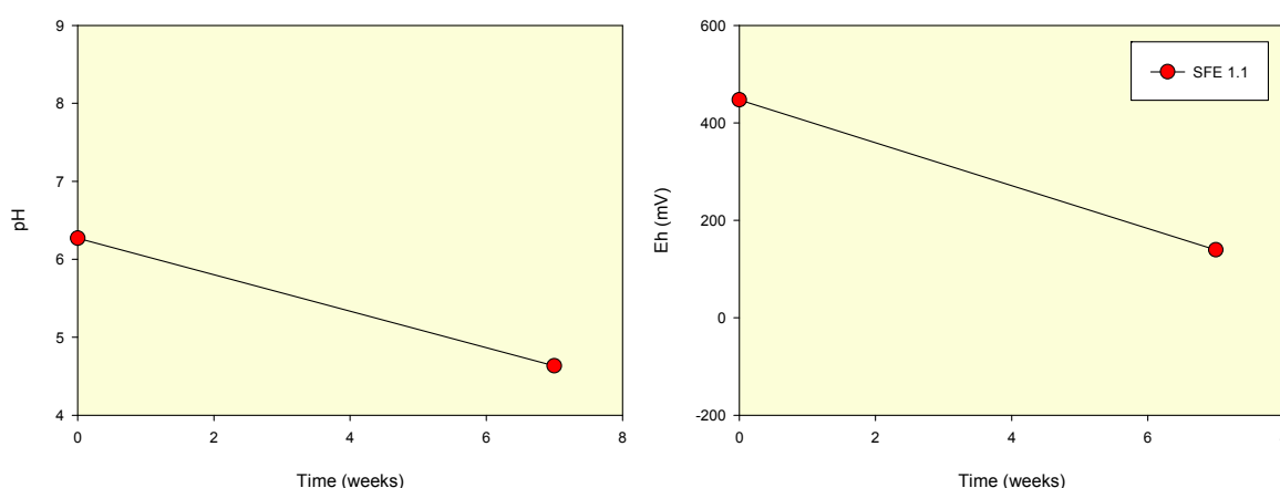
Figure 3-5 pH and Eh dynamics during monosulfide formation potential tests in surface soil sample SFE 1.1 from Swan Reach Ferry wetland.
