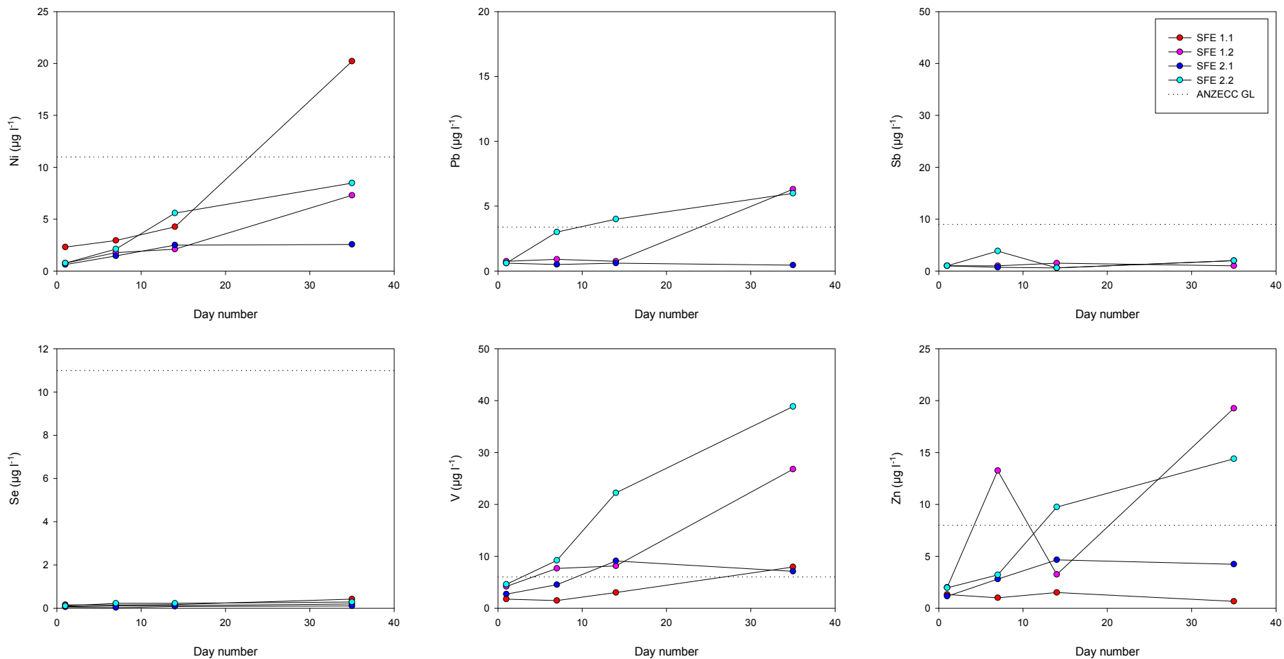
Figure 3-3 Contaminant and metalloid dynamics results for Swan Reach Ferry wetland soil materials for nickel (Ni), lead (Pb), antimony (Sb), selenium (Se), vanadium (V) and zinc (Zn).
