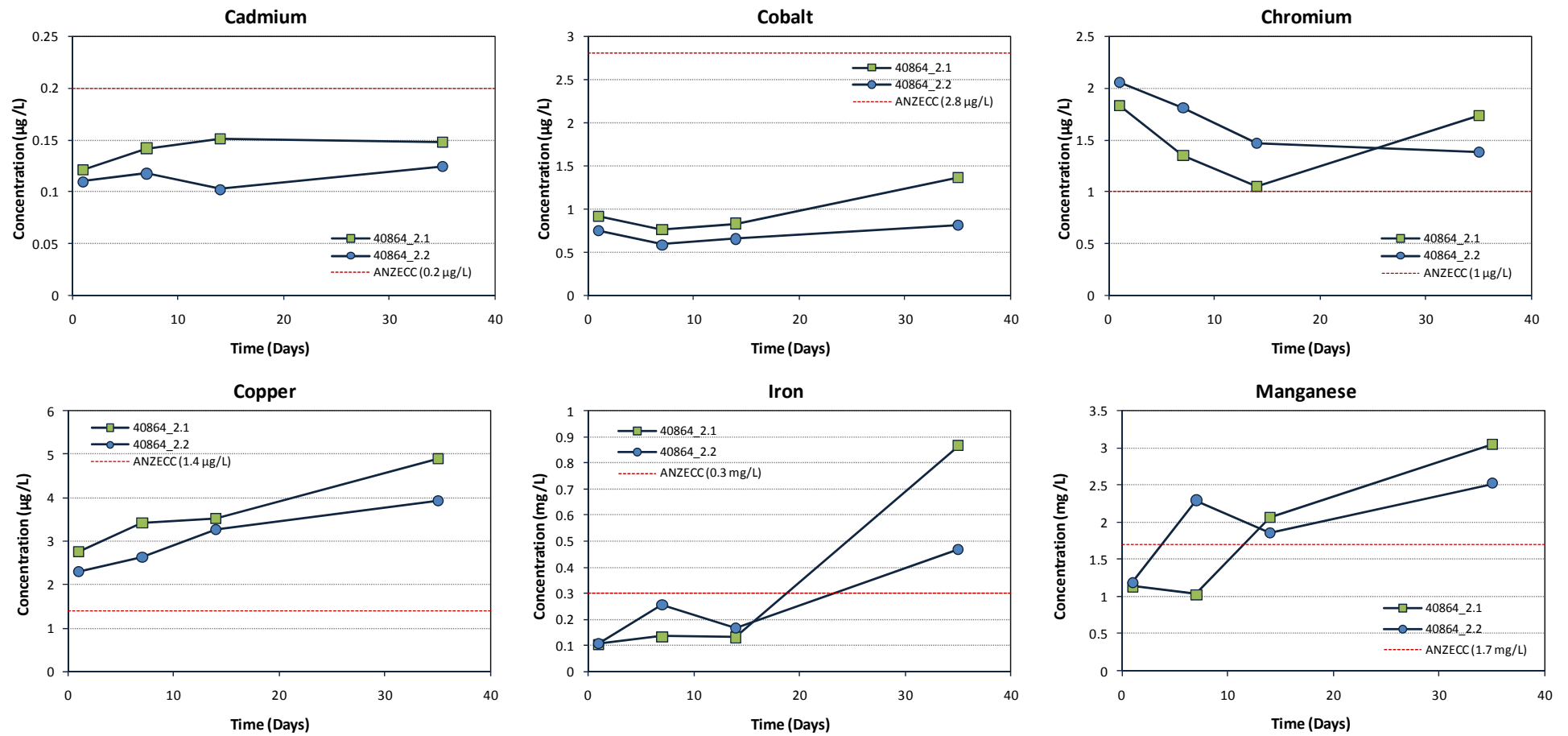
Figure 3-3: Contaminant and metalloid dynamics (Cd, Co, Cr, Cu, Fe and Mn) over 35 days for the Brickworks Lagoon soil materials (40864_2.1 and 40864_2.2).
